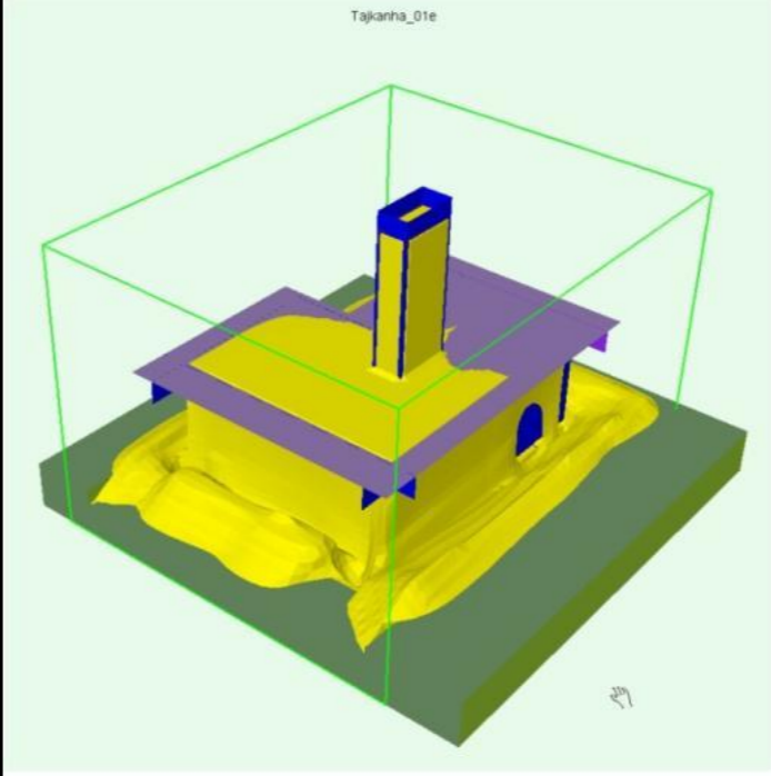
Figure 3: the yellow volumes represent air below 32 °C (ambient temperature = 40 °C)
